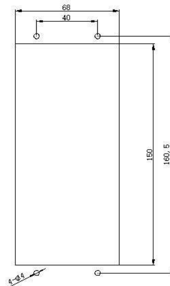
Cut-out Dimension
