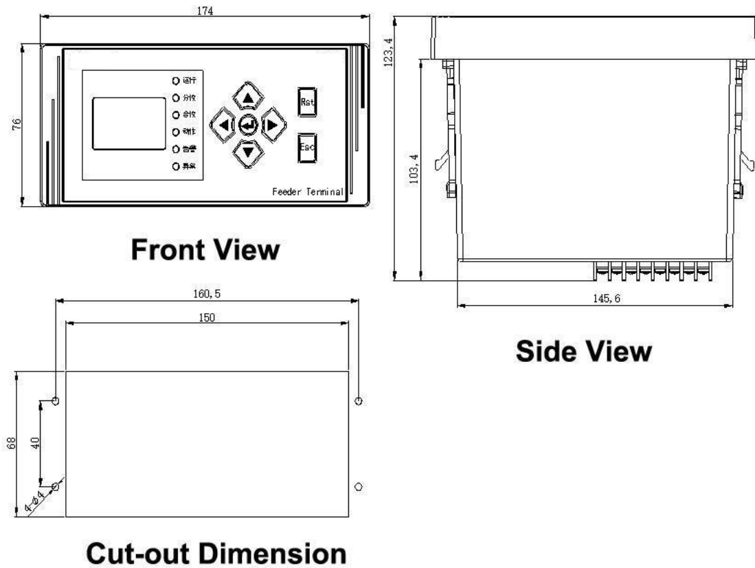
Fig. 4.2 VKRV-VI-H Dimensions and cut-out dimensions
